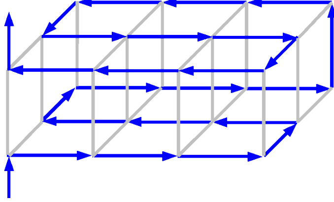
FIGURE 2. The alternating lexicographic order
